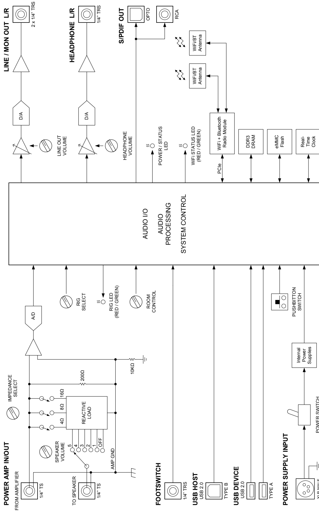
OX Amp Top Box Hardware Block Diagram
