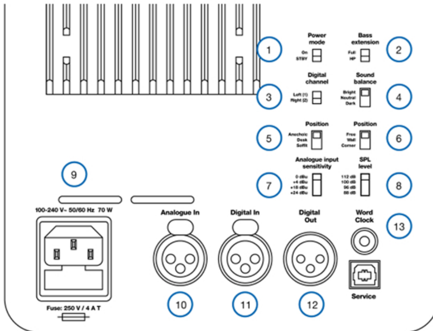
Figure 1: Core controls
