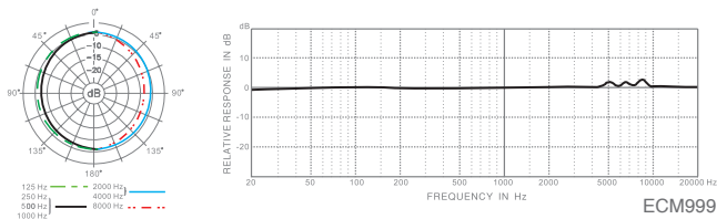
ECM999 Frequency Response (Omni)
