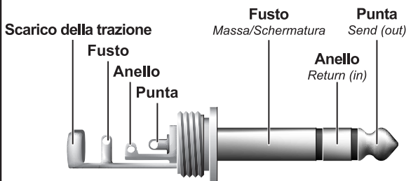
Fig. 5.7: Presse jack stereo Insert-Send-Return
